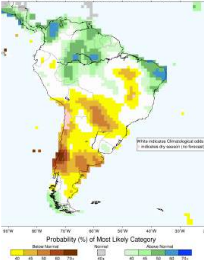
IRI Multi-Model Probability Forecast for Precipitation for June–July–August 2022, Issued May 2022
