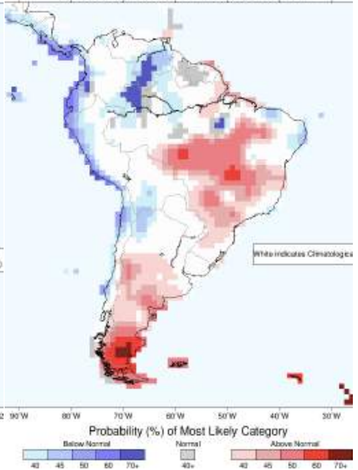
IRI Multi-Model Probability Forecast for Temperature for June–July–August 2022, Issued May 2022
