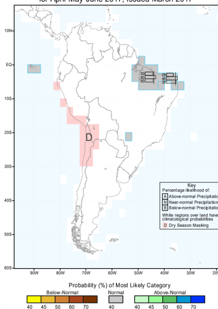
IRI Multi-Model Probability Forecast for Precipitation for April-May-June 2017, Issued March 2017
