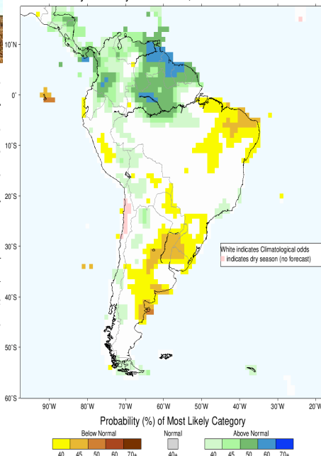
IRI Multi-Model Probability Forecast for Precipitation for January-February-March 2018, Issued December 2017
