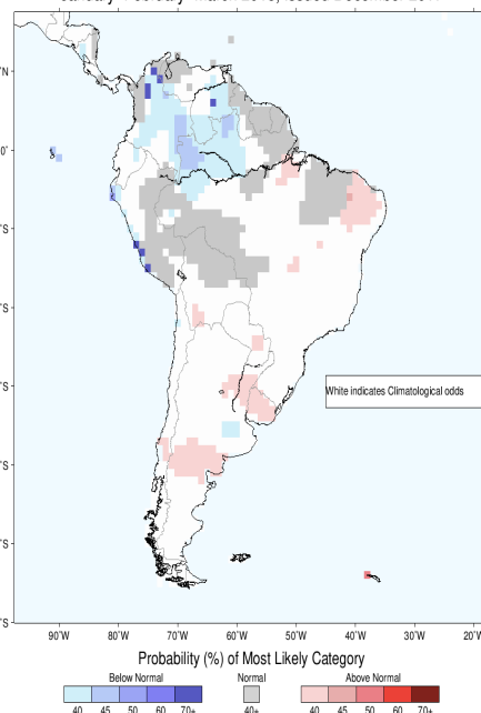
IRI Multi-Model Probability Forecast for Temperature for January-February-March 2018, Issued December 2017
